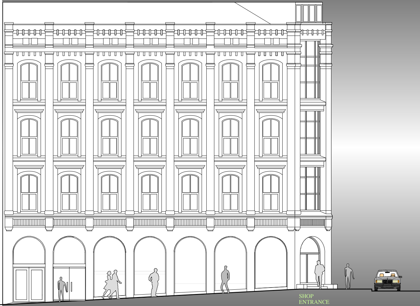
ELEVATION KARL JOHANS GATE
